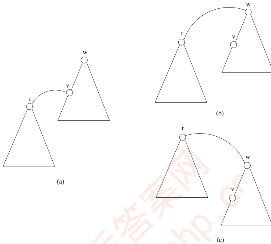
Figure 5: (a) The tree before GRAFT( r, v ). The cases on the right show the tree after GRAFT( r, v ) and the two cases: (b) \text{rank}(r) \leq \text{rank}(w) (c) \text{rank}(r) > \text{rank}(w)
