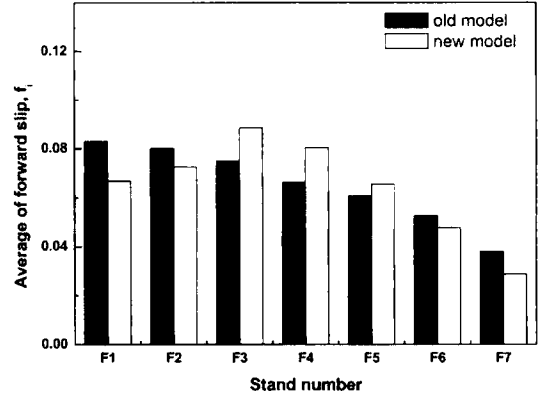
Fig. 4 Predicted forward slip at each stand
