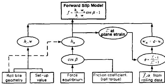
Fig. 6 Summary of forward slip calculation
