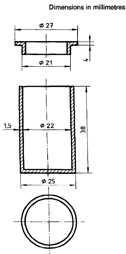
Figure 2 — Silica crucible and lid
