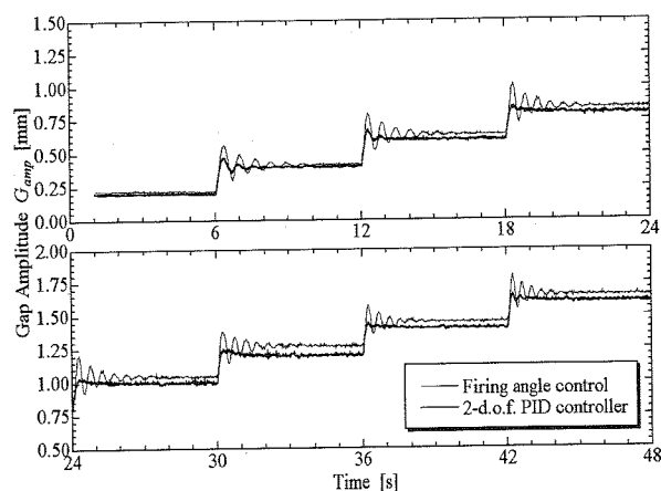
Fig. 16 Stepresponses with 2-d.o.f. controller
