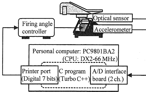
Fig. 6 Experimental system
