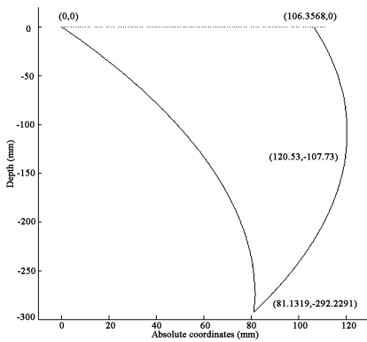
图 6 植树机坑形分析 ( v_{油缸} = 100\text{mm/s} ) Fig 6 Analysis on pit-shape of the planting tree machine ( v_{oilcylinder} = 100\text{mm/s} )
