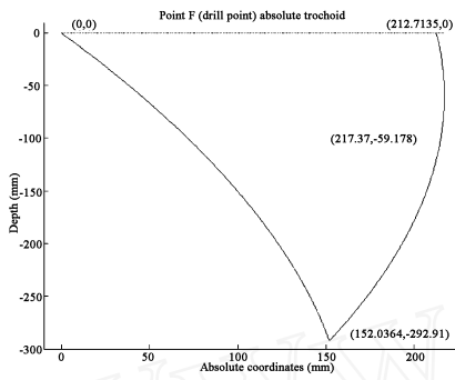
图 4 植树机坑形分析 ( v_{油缸} = 50\text{mm/s} ) Fig 4 Analysis on pit-shape of the planting tree machine ( v_{oilcylinder} = 50\text{mm/s} )
