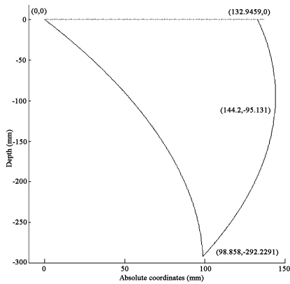
图 5 植树机坑形分析 ( v_{油缸} = 80\text{mm/s} ) Fig 5 Analysis on pit-shape of the planting tree machine ( v_{oilcylinder} = 80\text{mm/s} )
